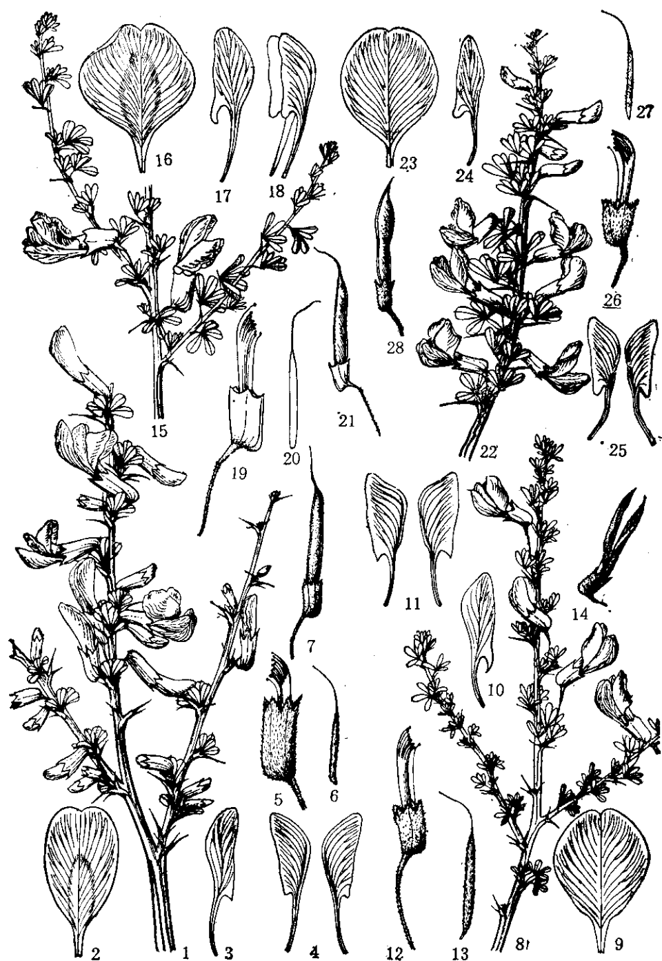
1—7.毛掌叶锦鸡儿 Caragana leveillei Kom.: 1.花枝, 2.旗瓣, 3.翼瓣, 4.龙骨瓣, 5.雄蕊和花萼, 6.雌蕊, 7.幼果。8—14.白毛锦鸡儿 C. licentiana Hand-Mazz.: 8.花枝, 9.旗瓣, 10.翼瓣, 11.龙骨瓣, 12.雄蕊和花萼, 13.雌蕊, 14.荚果(裂开)。15—21.甘蒙锦鸡儿 C. opulens Kom.: 15.花枝, 16.旗瓣, 17.翼瓣, 18.龙骨瓣, 19.雄蕊和花萼, 20.雌蕊, 21.荚果。22—28.昆仑锦鸡儿 C. polourensis Franch.: 22.花枝, 23.旗瓣, 24.翼瓣, 25.龙骨瓣, 26.雄蕊和花萼, 27.雌蕊, 28.荚果。(蔡淑琴绘)
